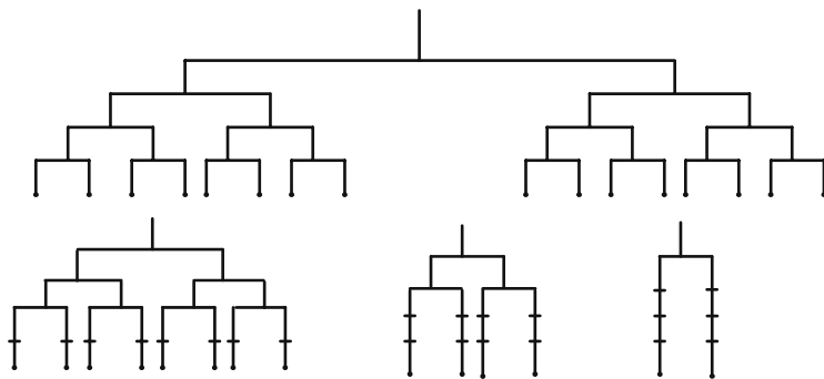
FIGURE 16.2 Anderson five-stage staggered nested design.
