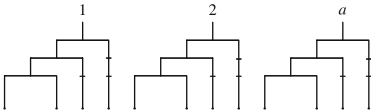
FIGURE 16.3 Bainbridge four-stage inverted nested design with a single replicate.
