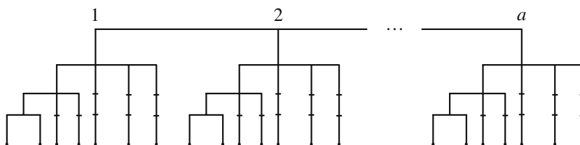
FIGURE 16.5 Heckler–Rao four-stage extended staggered design.
